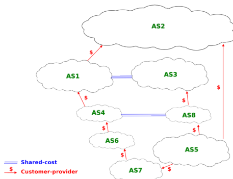
Figure 5.68: Asymmetry of Internet paths
