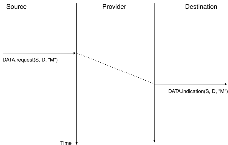
Figure 2.14: A simple connectionless service
