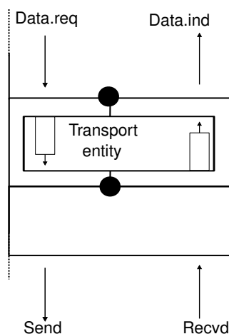
Figure 4.1: Interactions between the transport layer, its user, and its network layer provider
