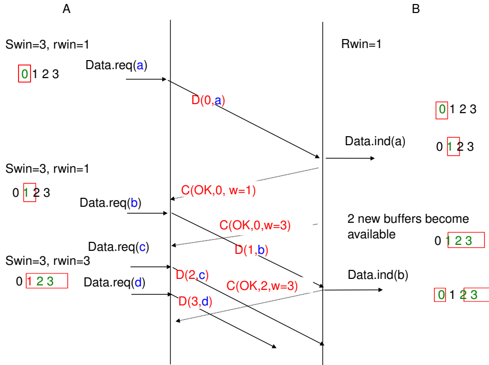
Figure 4.19: Dynamic receiving window
