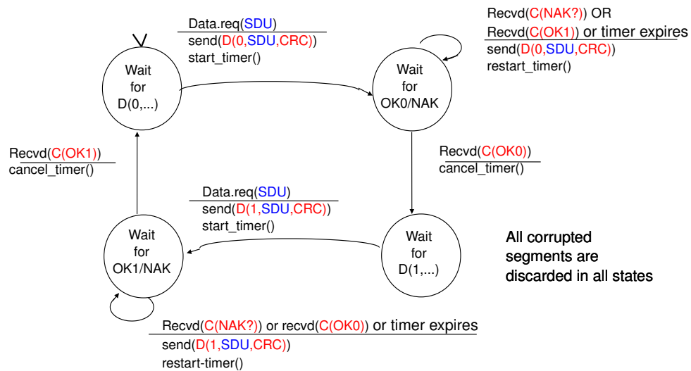
Figure 4.7: Alternating bit protocol : Sender FSM
