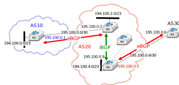
Figure 5.65: How to deal with non-BGP routers ?
