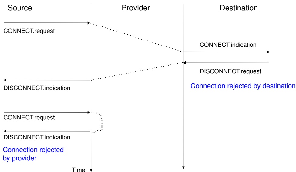
Figure 2.22: Two types of rejection for a connection establishment attempt
