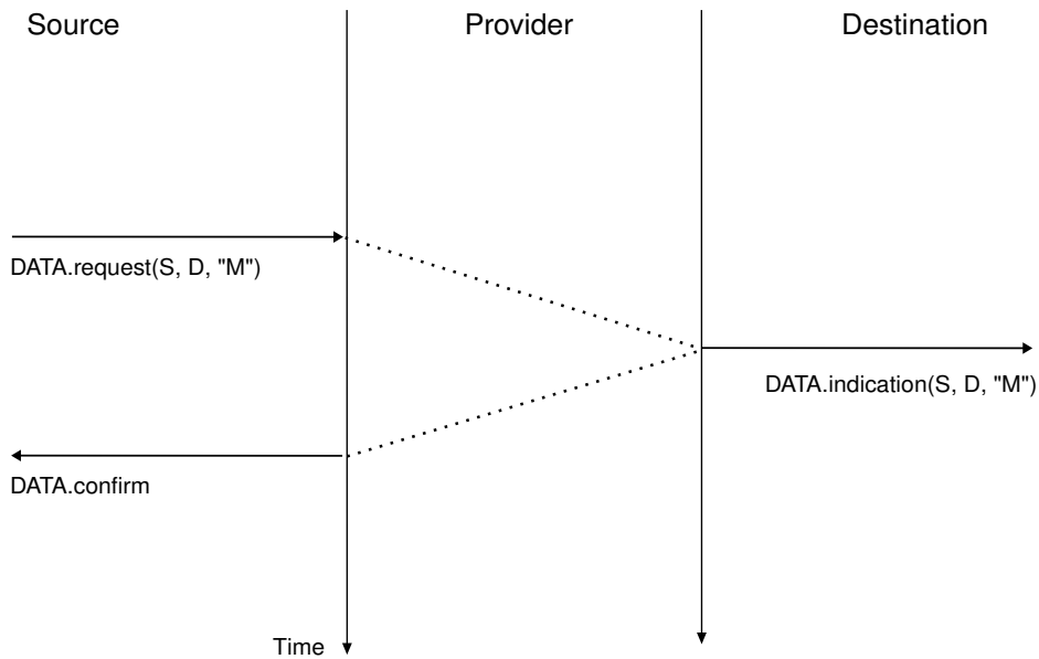
Figure 2.20: A confirmed connectionless service
