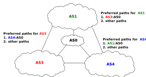
Figure 5.72: The bad gadget internetwork
