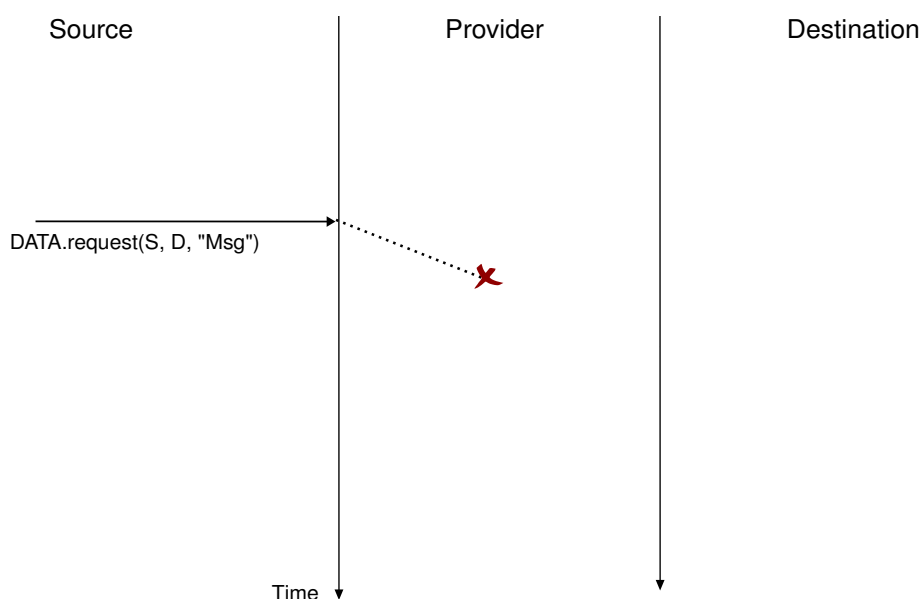
Figure 2.15: An unreliable connectionless service may lose SDUs
