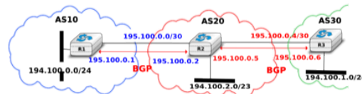
Figure 5.62: Utilisation of the BGP nexthop attribute
