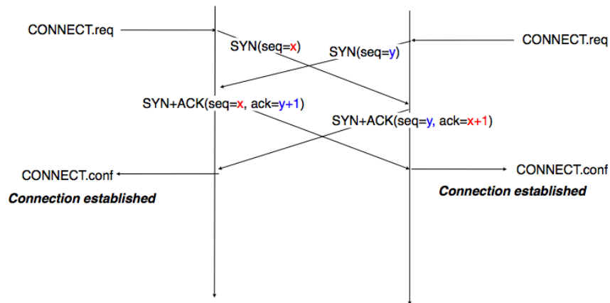
Figure 4.40: Simultaneous establishment of a TCP connection
