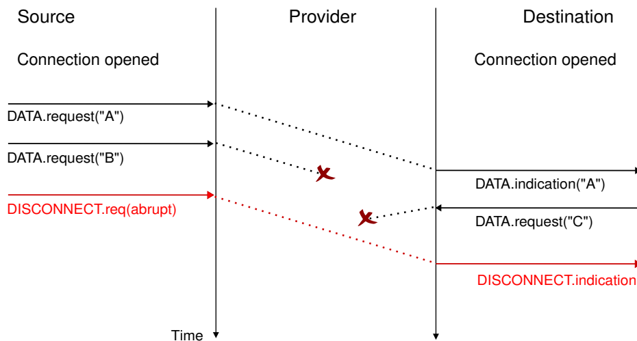
Figure 2.26: Abrupt connection release initiated by a user
