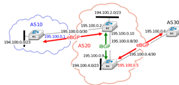
Figure 5.64: iBGP and eBGP sessions
