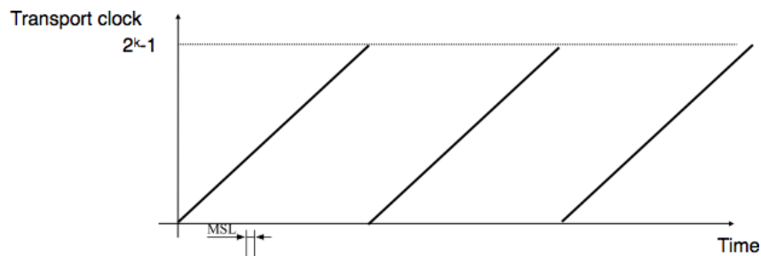
Figure 4.26: Transport clock
