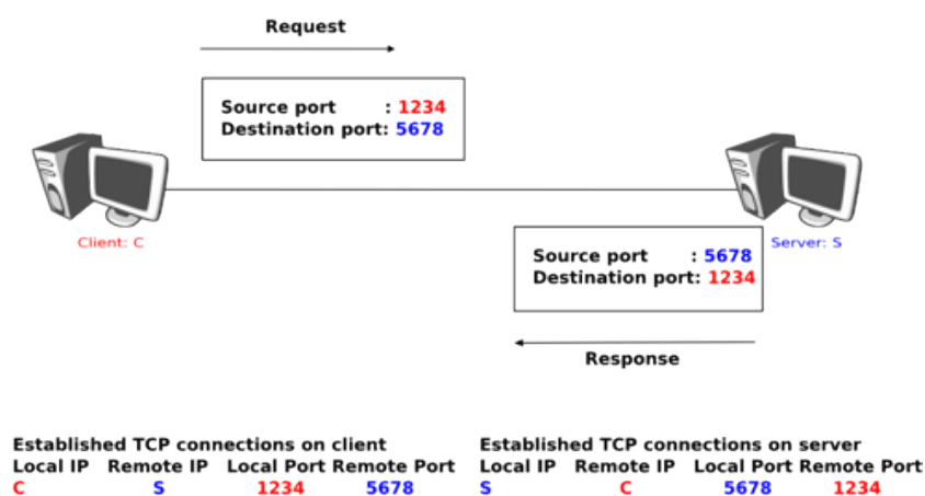
Figure 4.36: Utilization of the TCP source and destination ports
