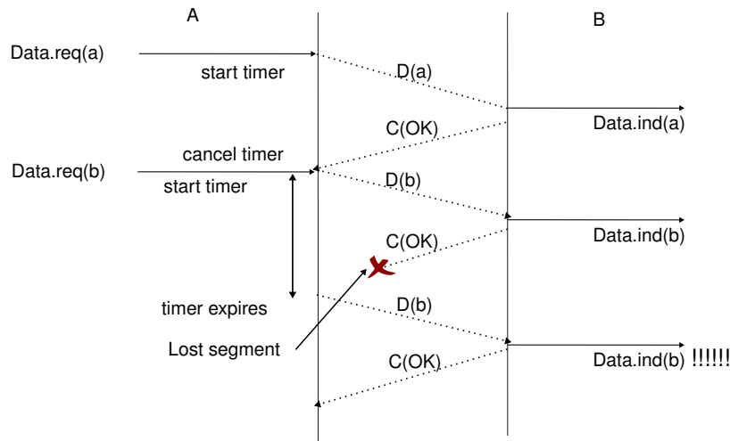
Figure 4.6: Limitations of retransmission timers
