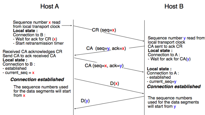
Figure 4.27: Three-way handshake
