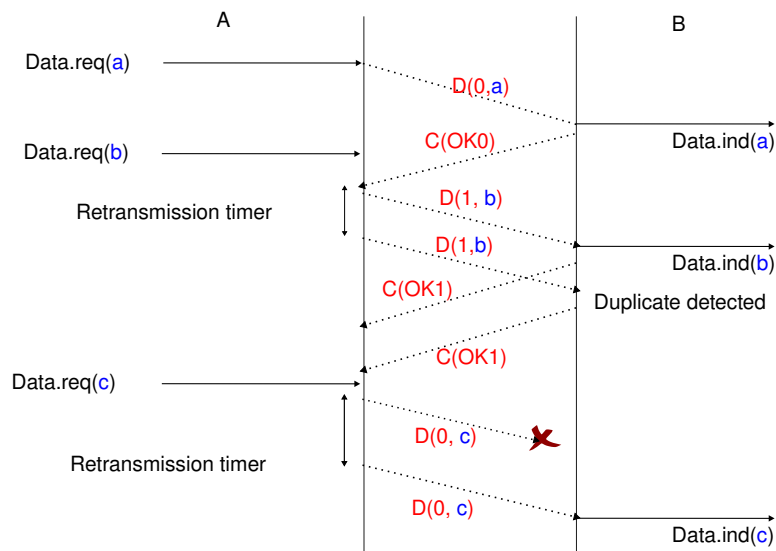
Figure 4.9: Operation of the alternating bit protocol
