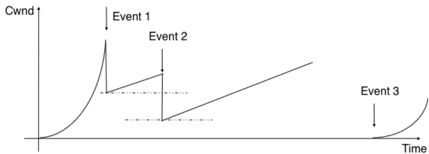
Figure 4.60: Evolution of the congestion window
