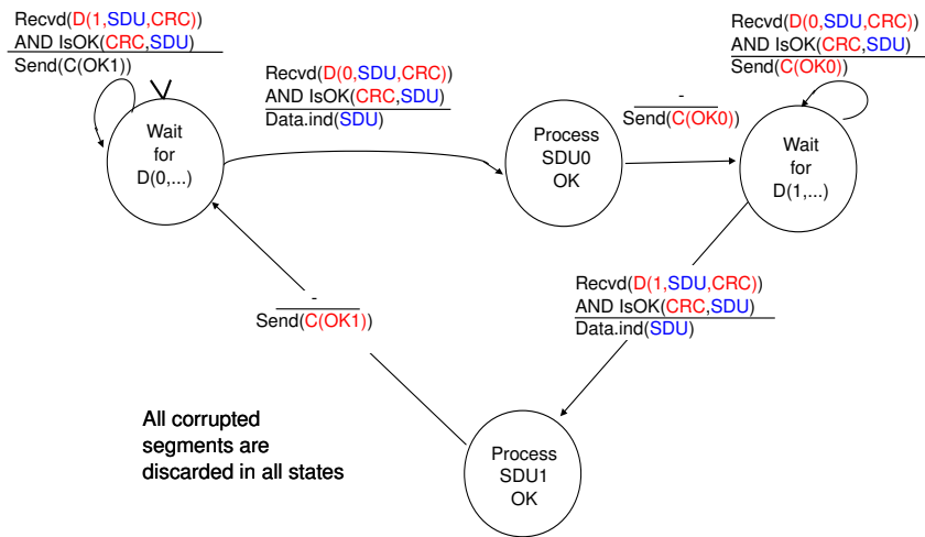
Figure 4.8: Alternating bit protocol : Receiver FSM
