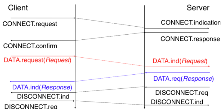
Figure 3.20: HTTP 1.0 and the underlying TCP connection
