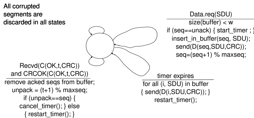
Figure 4.15: Go-back-n : sender FSM
