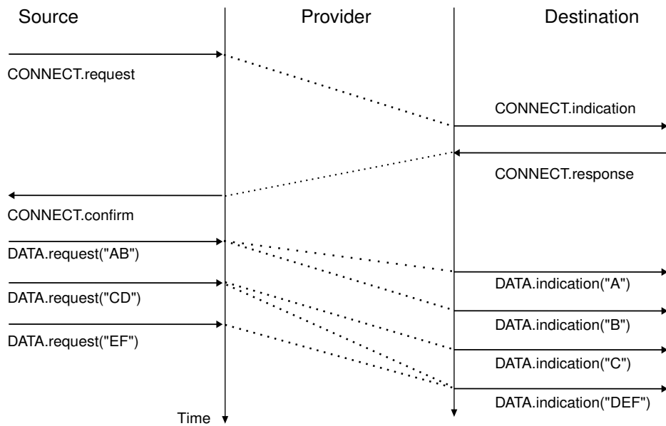
Figure 2.24: Stream-mode transfer in a connection oriented service
