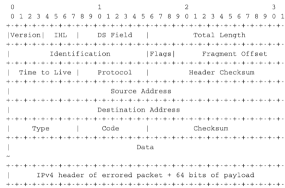
Figure 5.31: ICMP version 4 (RFC 792)
