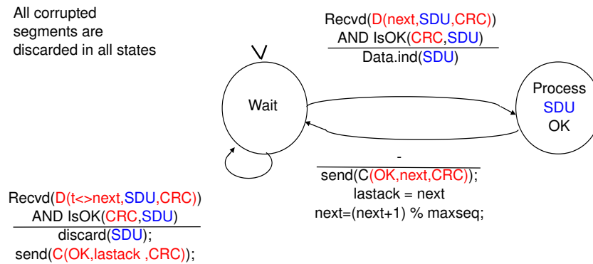
Figure 4.14: Go-back-n : receiver FSM
