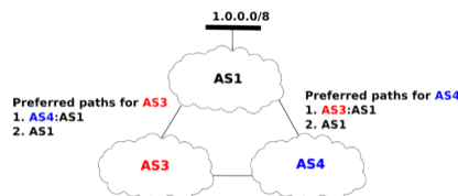
Figure 5.71: The disagree internetwork
